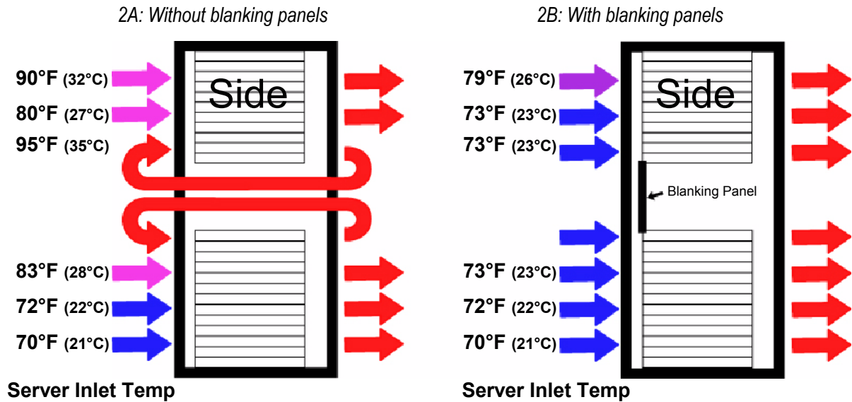
Figure 3 – Effect of installation of blanking panel on server air inlet temperature
